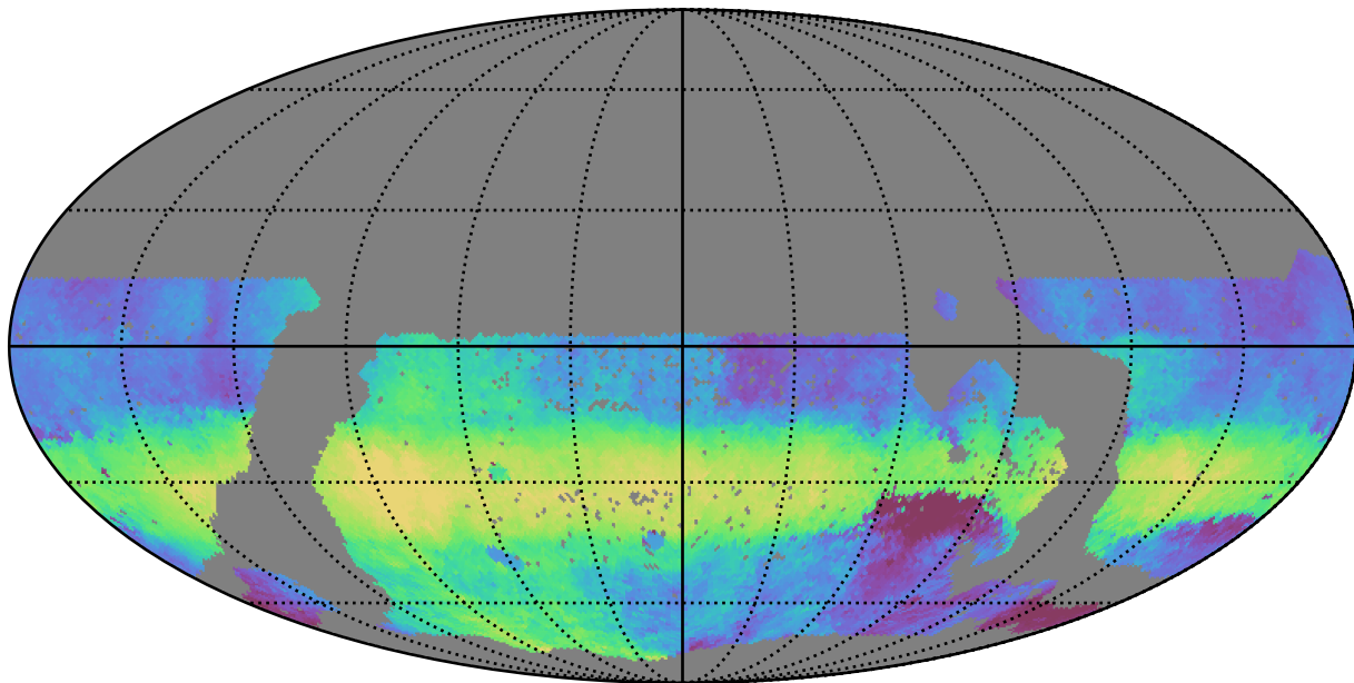
mw_roll_all_v3.3_10yrs WFD r band: Median HA
