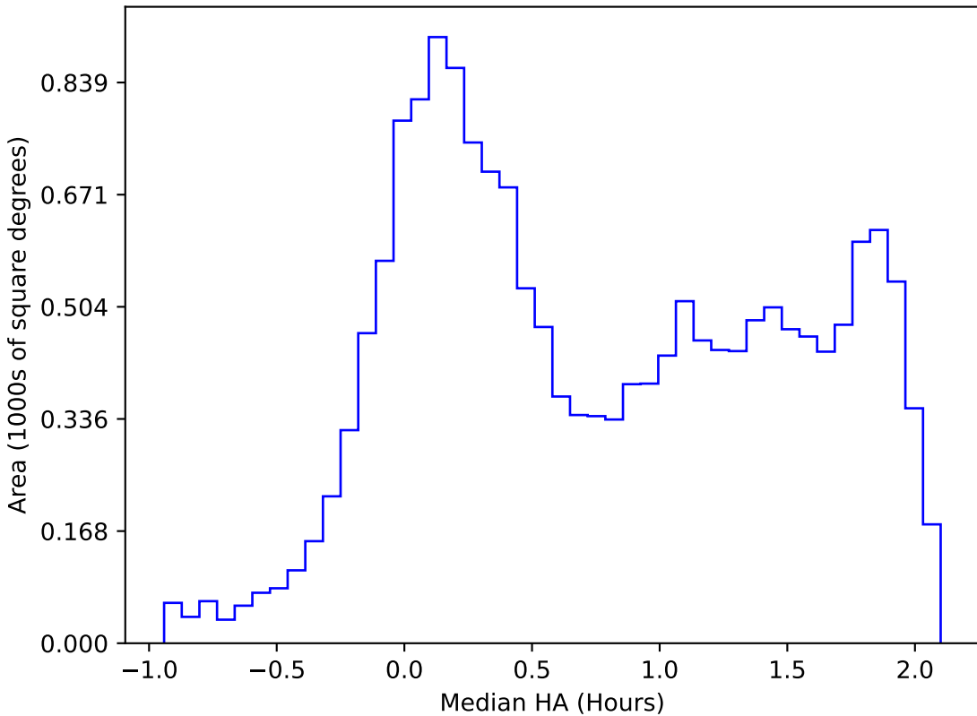
mw_roll_all_v3.3_10yrs WFD r band: Median HA
