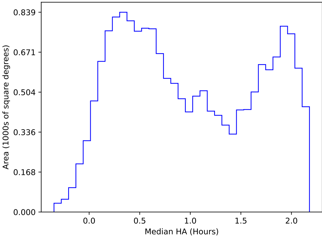
mw_roll_all_v3.3_10yrs WFD i band: Median HA
