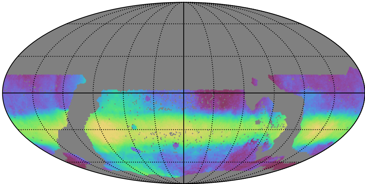
mw_roll_all_v3.3_10yrs WFD all bands: Median HA
