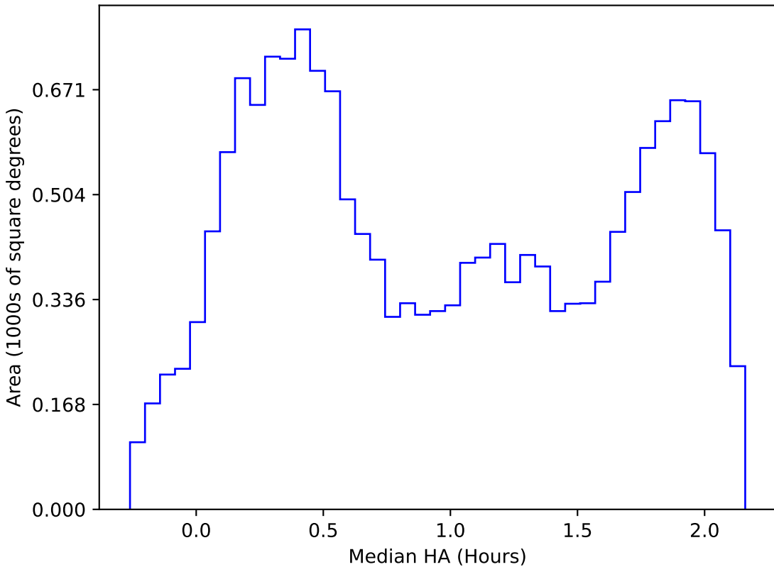
mw_roll_all_v3.3_10yrs WFD all bands: Median HA
