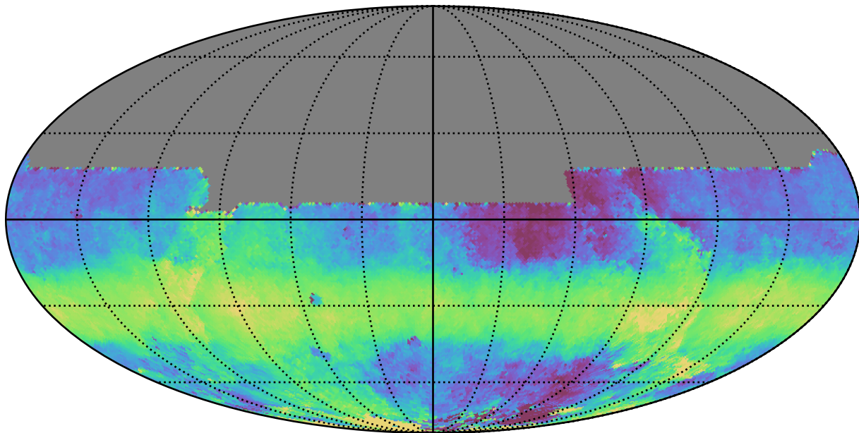
mw_roll_all_v3.3_10yrs All sky y band: Median HA
