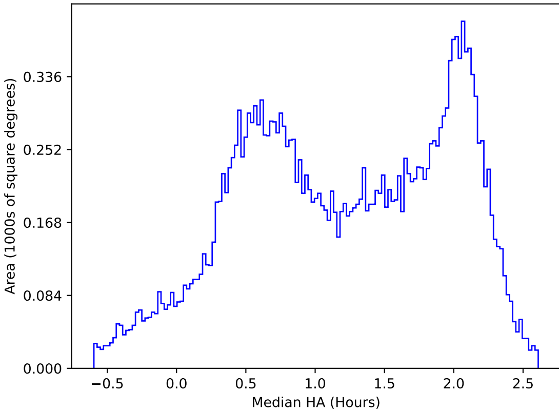
mw_roll_all_v3.3_10yrs All sky y band: Median HA
