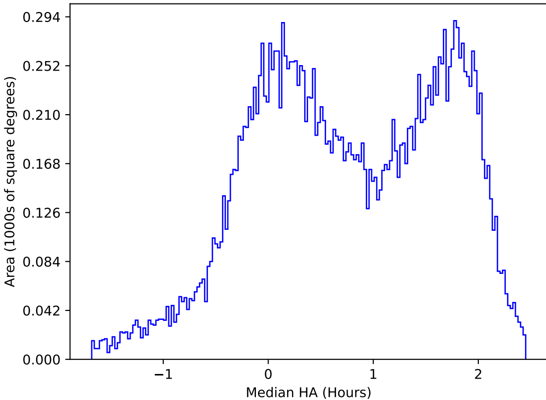
mw_roll_all_v3.3_10yrs All sky u band: Median HA
