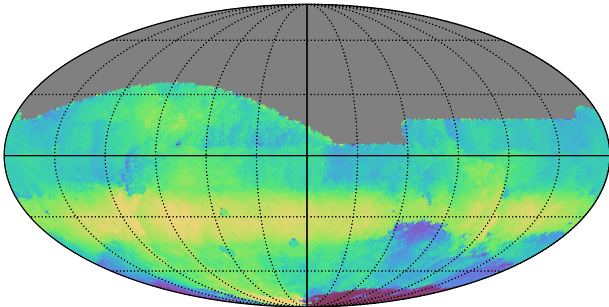
mw_roll_all_v3.3_10yrs All sky r band: Median HA
