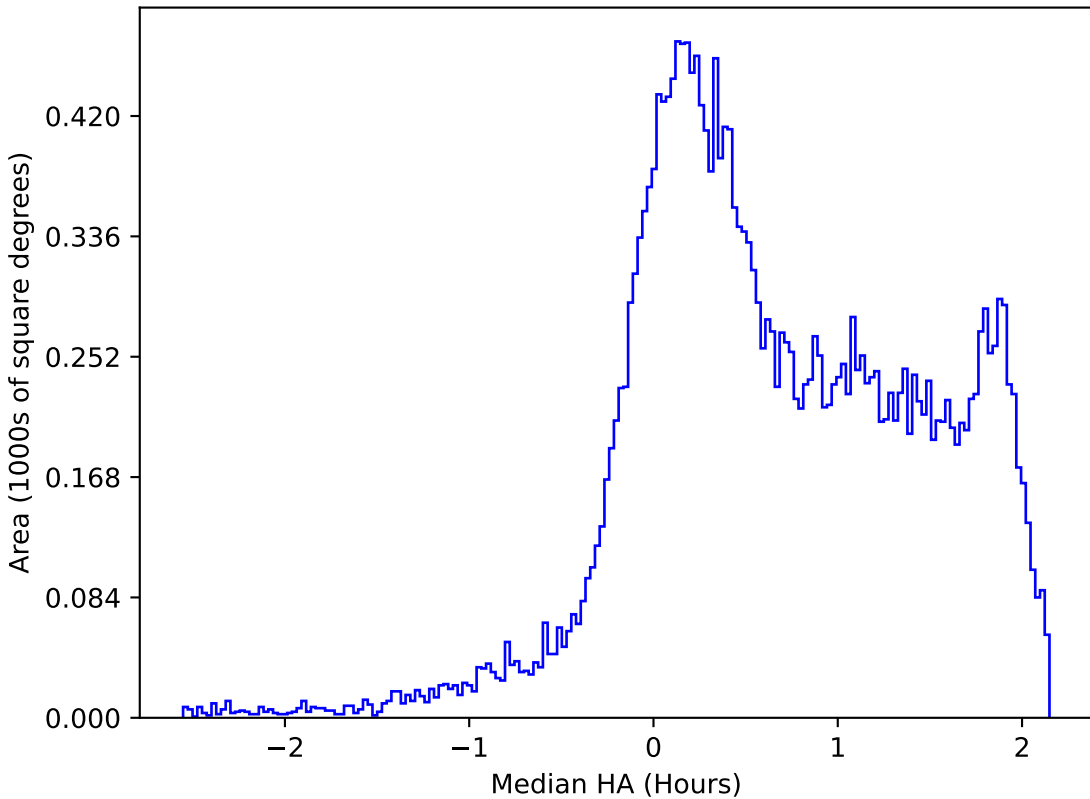
mw_roll_all_v3.3_10yrs All sky r band: Median HA
