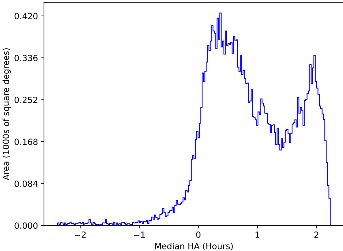
mw_roll_all_v3.3_10yrs All sky i band: Median HA
