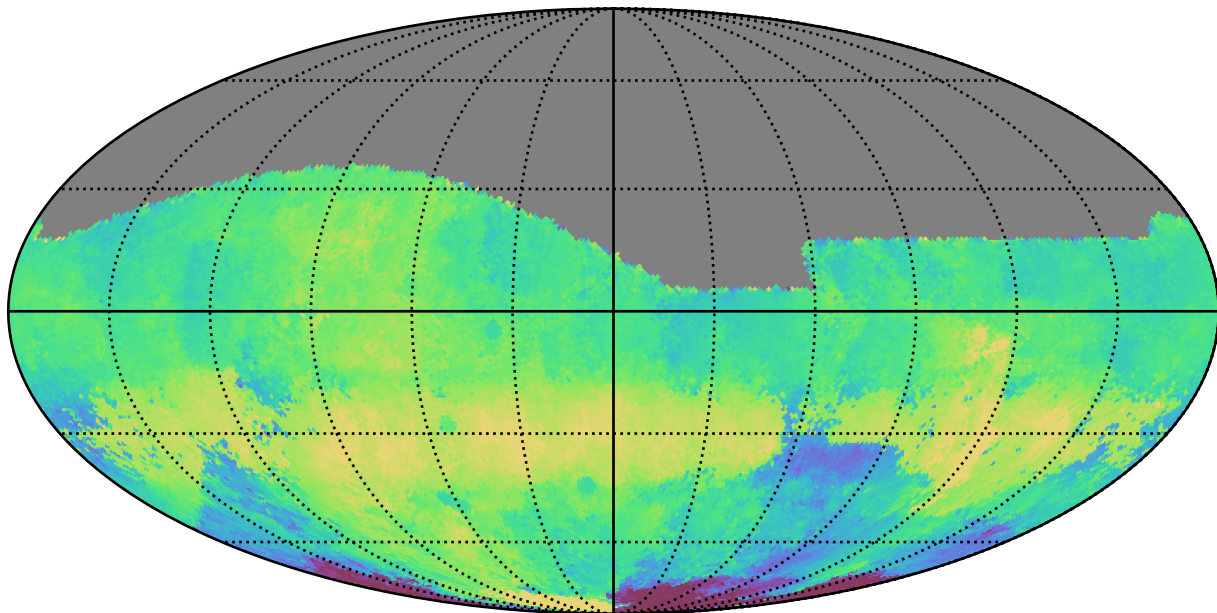
mw_roll_all_v3.3_10yrs All sky g band: Median HA
