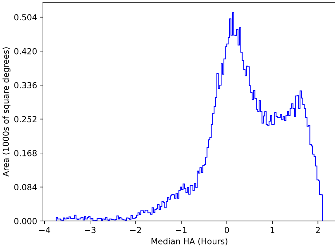
mw_roll_all_v3.3_10yrs All sky g band: Median HA
