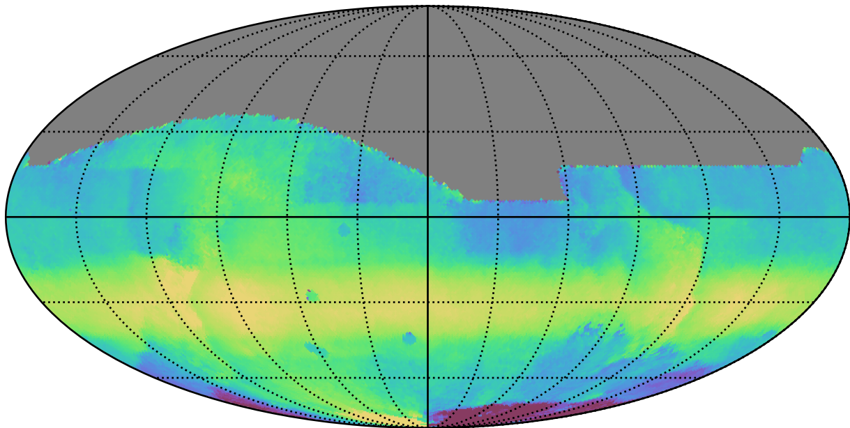
mw_roll_all_v3.3_10yrs All sky all bands: Median HA
