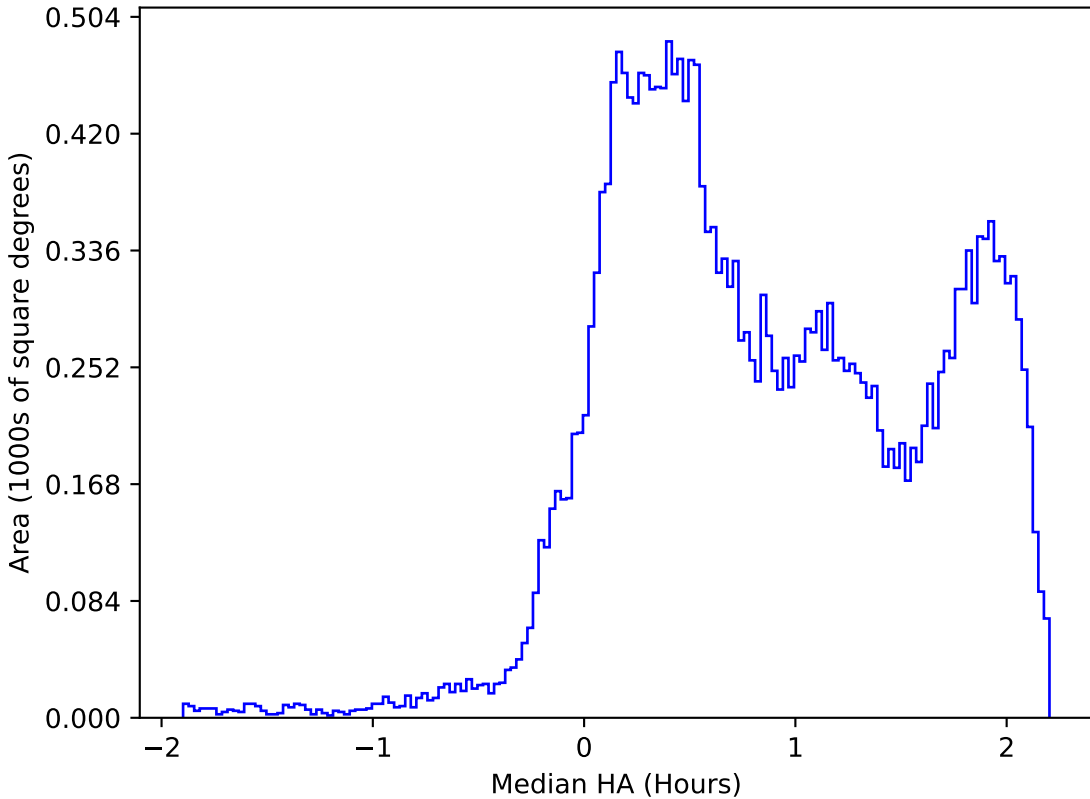
mw_roll_all_v3.3_10yrs All sky all bands: Median HA
