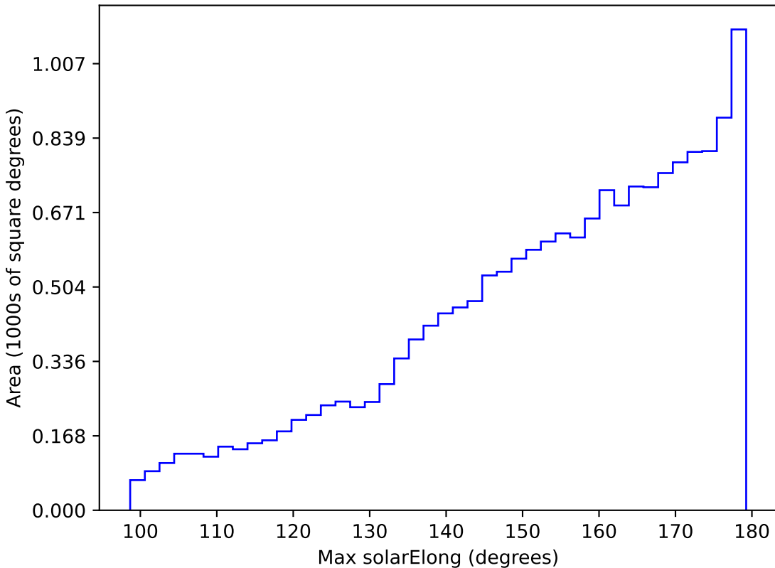
mw_roll_all_v3.3_10yrs WFD z band: Max solarElong
