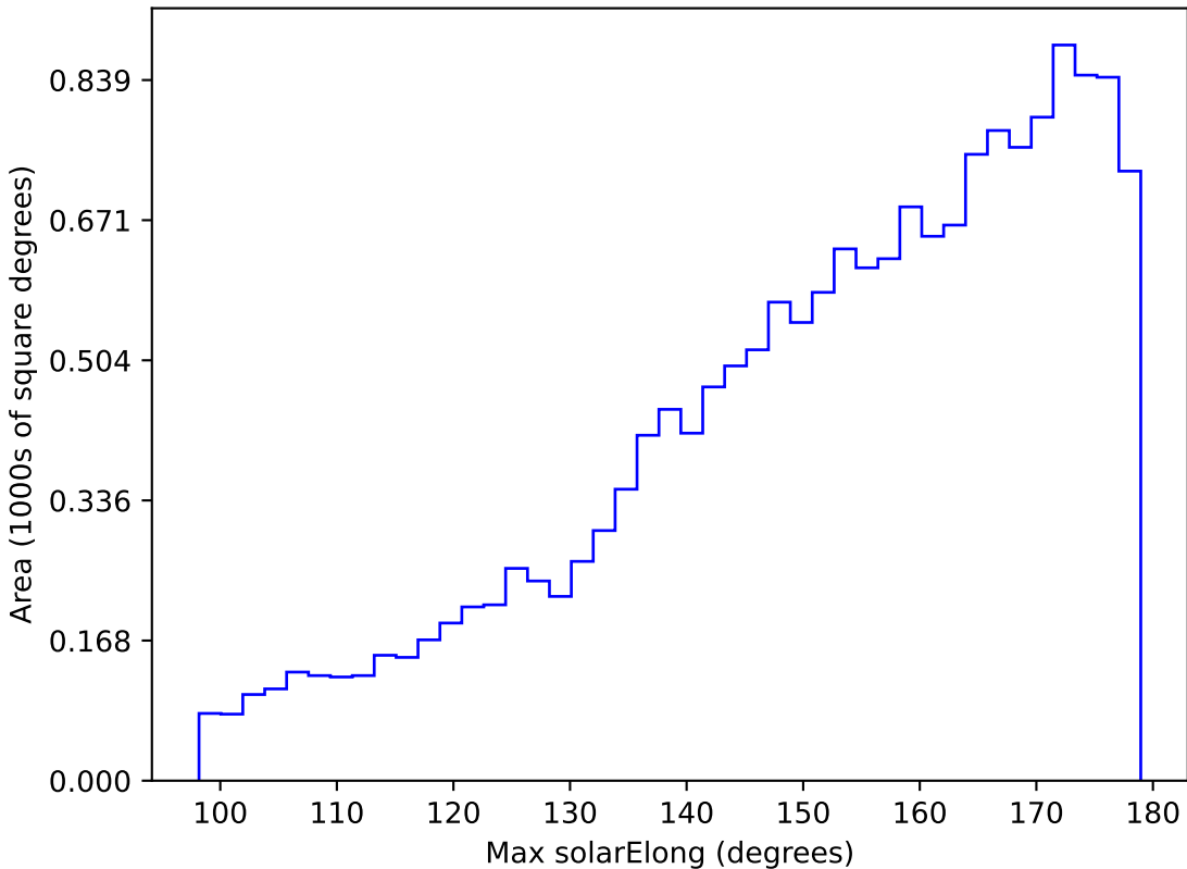
mw_roll_all_v3.3_10yrs WFD u band: Max solarElong
