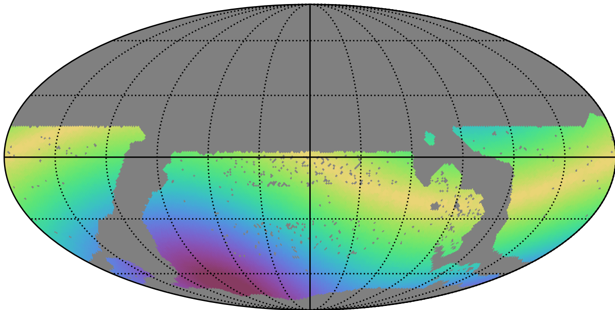
mw_roll_all_v3.3_10yrs WFD r band: Max solarElong
