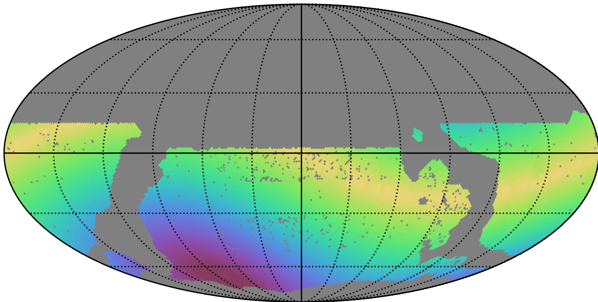
mw_roll_all_v3.3_10yrs WFD g band: Max solarElong
