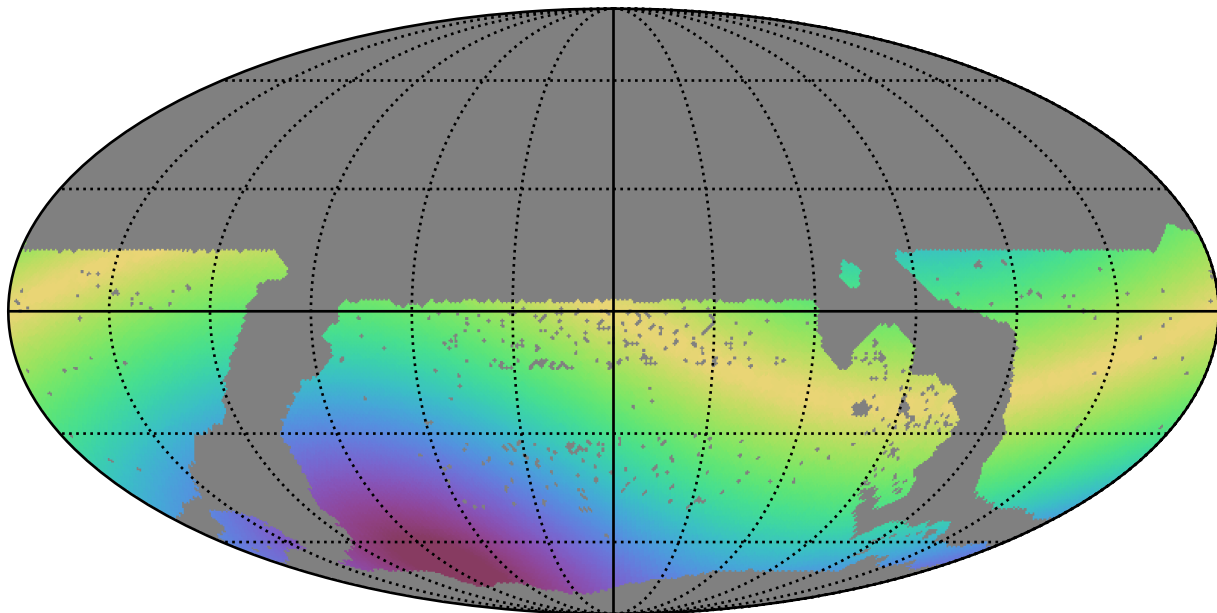
mw_roll_all_v3.3_10yrs WFD all bands: Max solarElong
