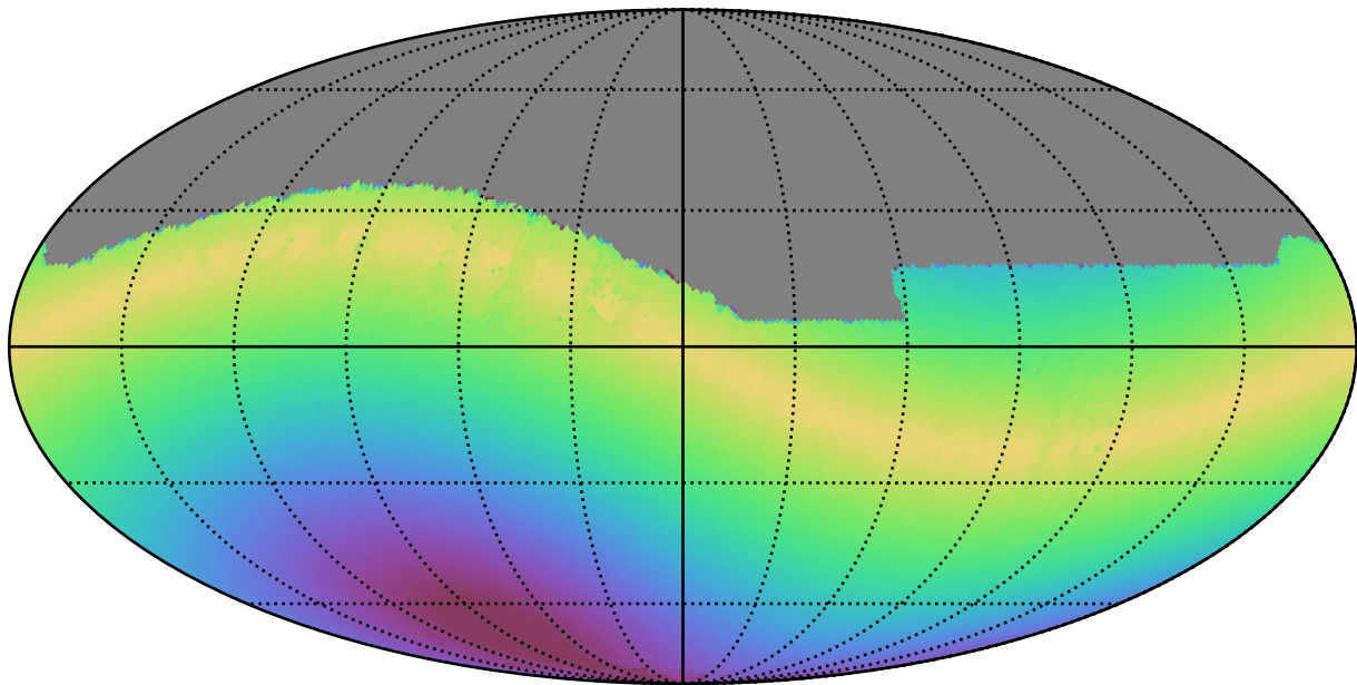
mw_roll_all_v3.3_10yrs All sky z band: Max solarElong
