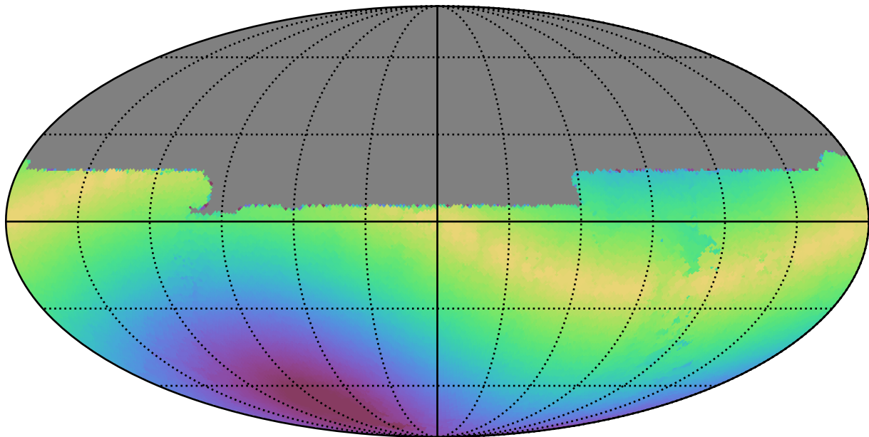
mw_roll_all_v3.3_10yrs All sky u band: Max solarElong
