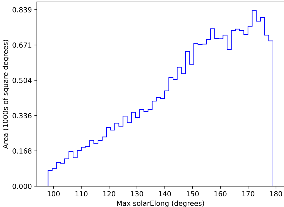
mw_roll_all_v3.3_10yrs All sky u band: Max solarElong
