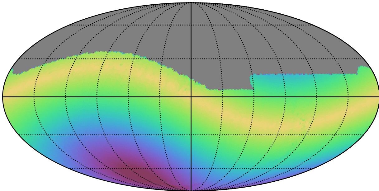
mw_roll_all_v3.3_10yrs All sky r band: Max solarElong
