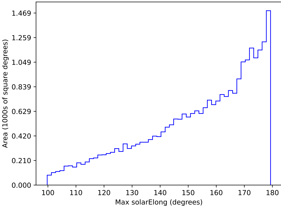
mw_roll_all_v3.3_10yrs All sky r band: Max solarElong
