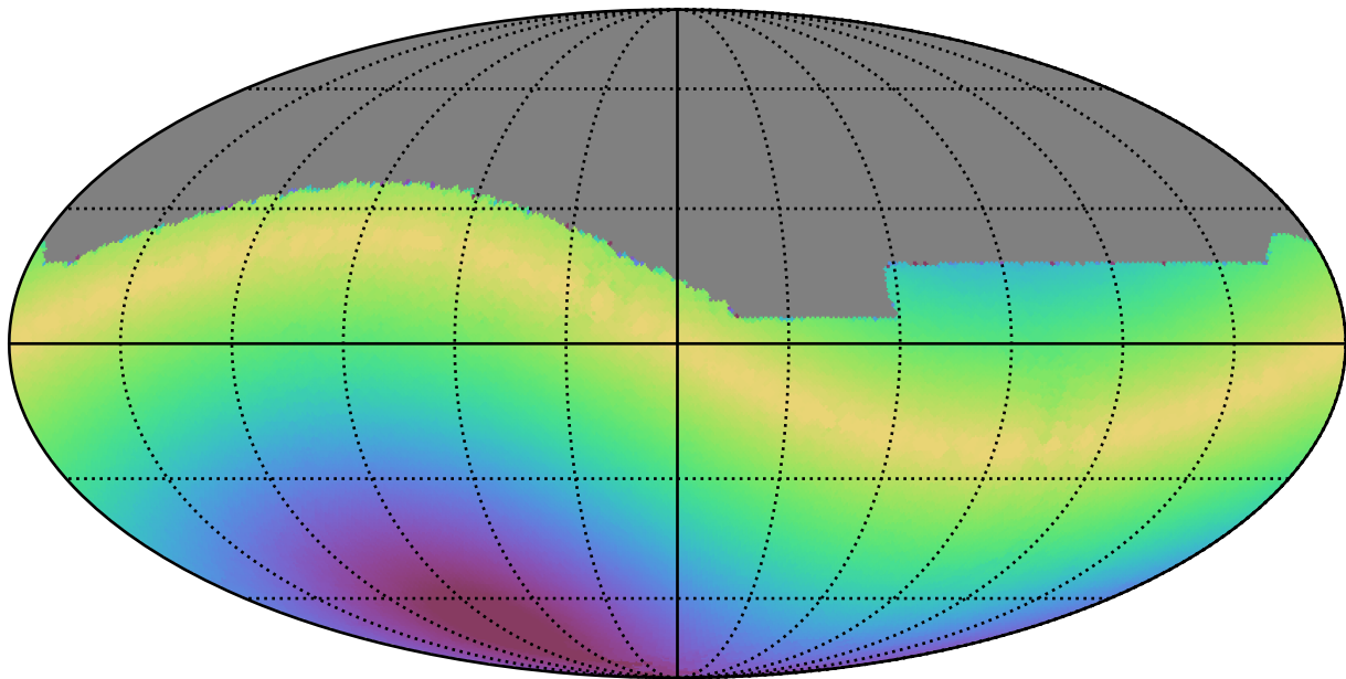
mw_roll_all_v3.3_10yrs All sky i band: Max solarElong
