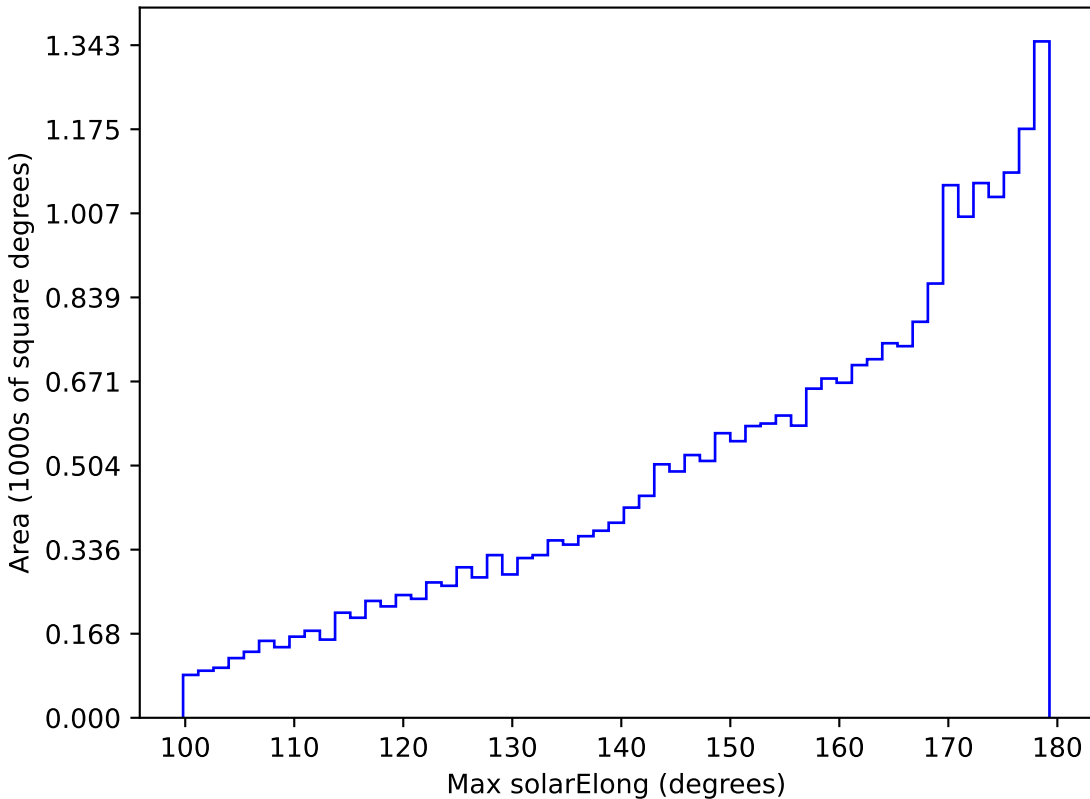
mw_roll_all_v3.3_10yrs All sky i band: Max solarElong
