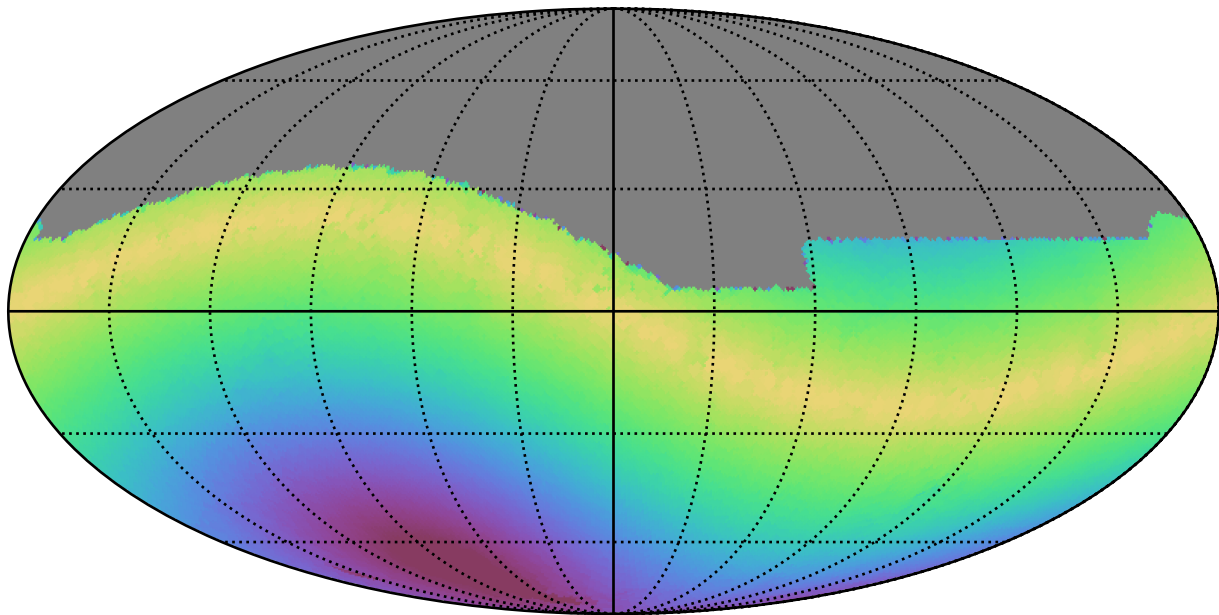
mw_roll_all_v3.3_10yrs All sky g band: Max solarElong
