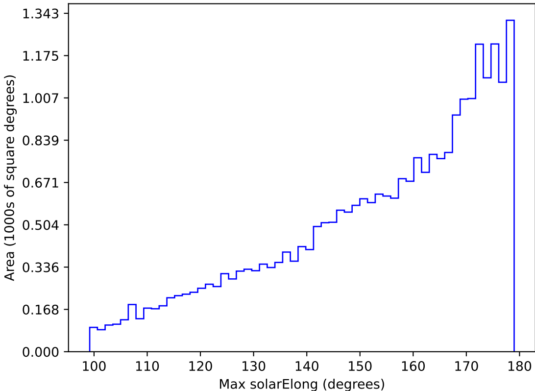
mw_roll_all_v3.3_10yrs All sky g band: Max solarElong
