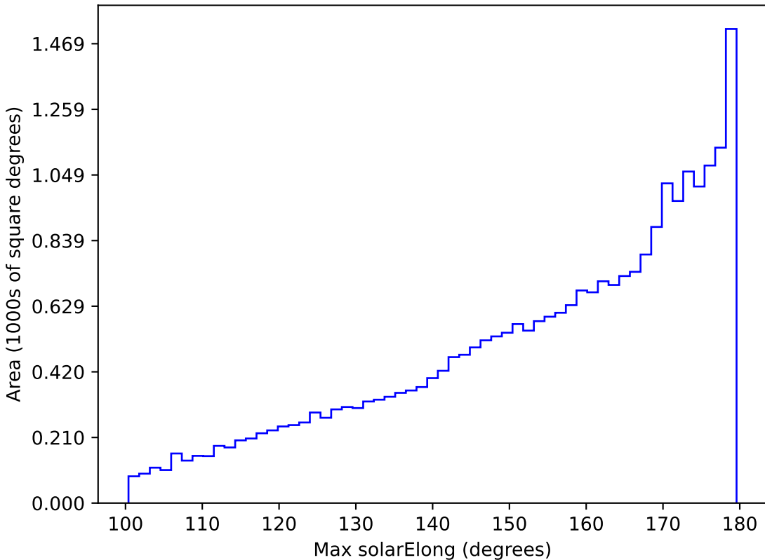
mw_roll_all_v3.3_10yrs All sky all bands: Max solarElong
