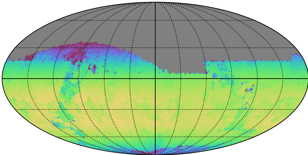
mw_roll_all_v3.3_10yrs Yr 1 z band: Max skyBrightness
