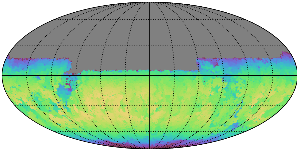
mw_roll_all_v3.3_10yrs Yr 1 y band: Max skyBrightness
