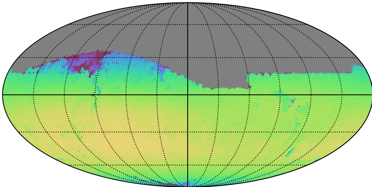
mw_roll_all_v3.3_10yrs Yr 1 i band: Max skyBrightness
