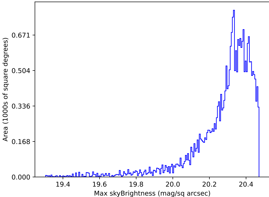
mw_roll_all_v3.3_10yrs Yr 1 i band: Max skyBrightness
