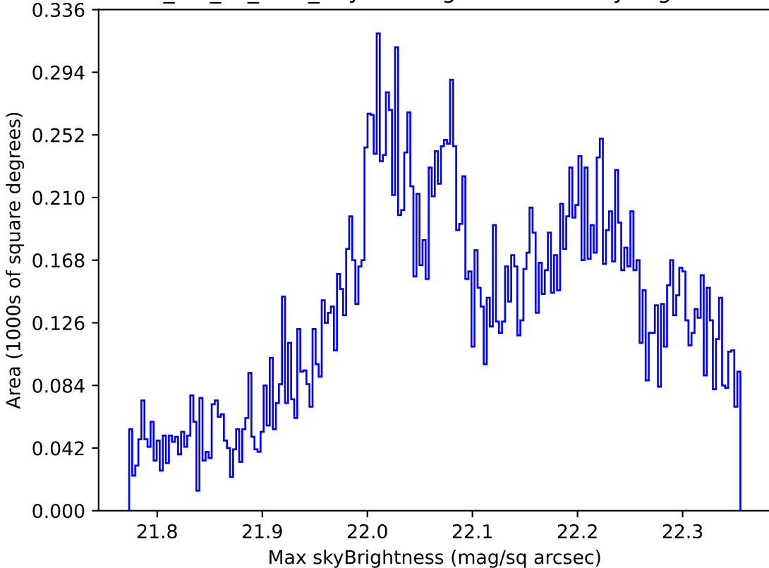
mw_roll_all_v3.3_10yrs Yr 1 g band: Max skyBrightness
