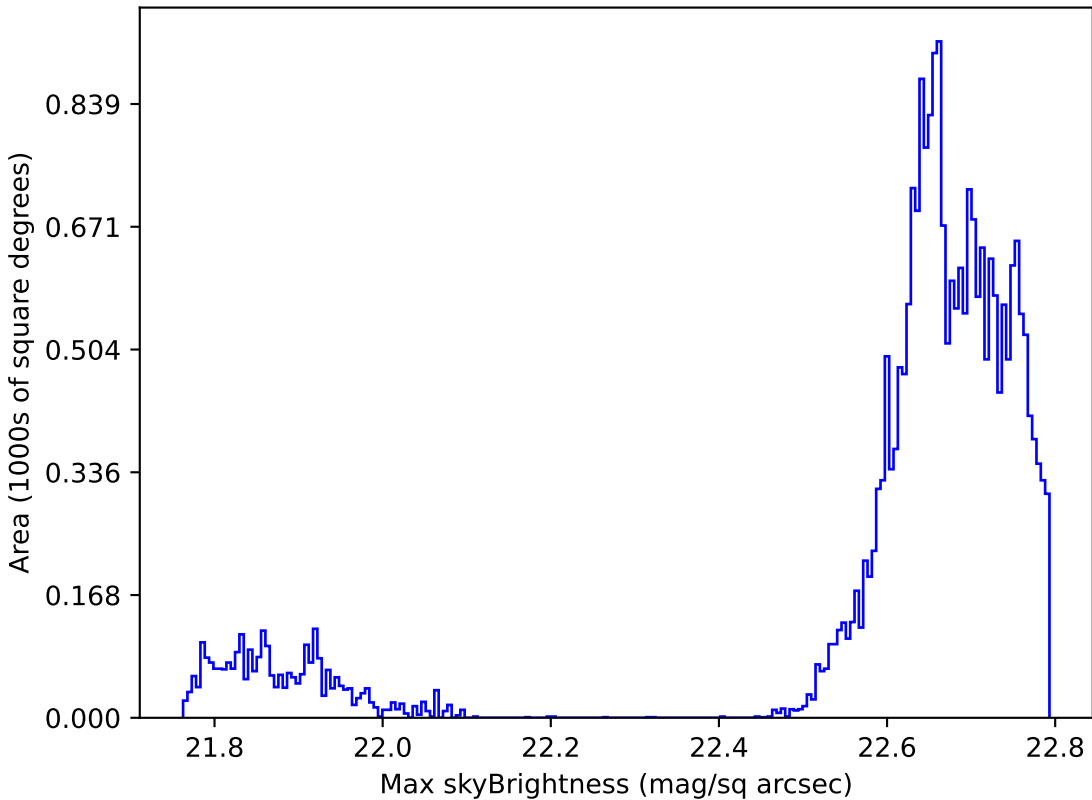
mw_roll_all_v3.3_10yrs Yr 1 all bands: Max skyBrightness
