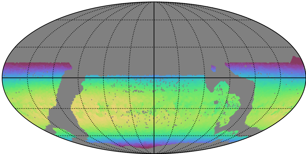
mw_roll_all_v3.3_10yrs WFD z band: Max skyBrightness
