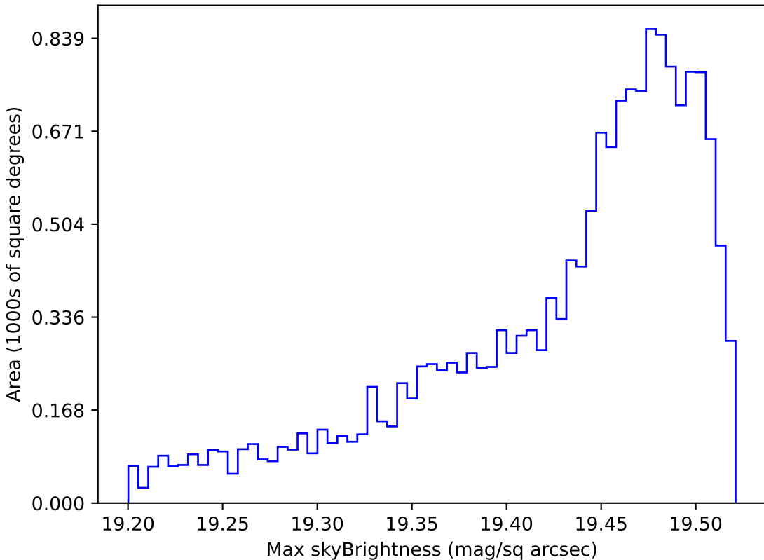
mw_roll_all_v3.3_10yrs WFD z band: Max skyBrightness
