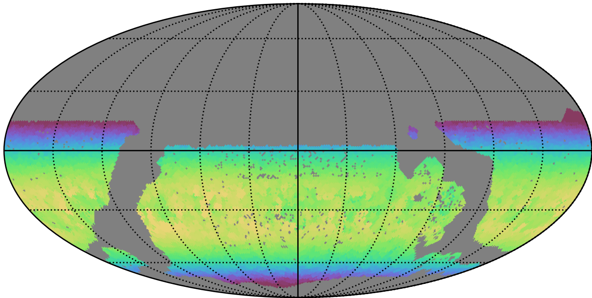
mw_roll_all_v3.3_10yrs WFD y band: Max skyBrightness
