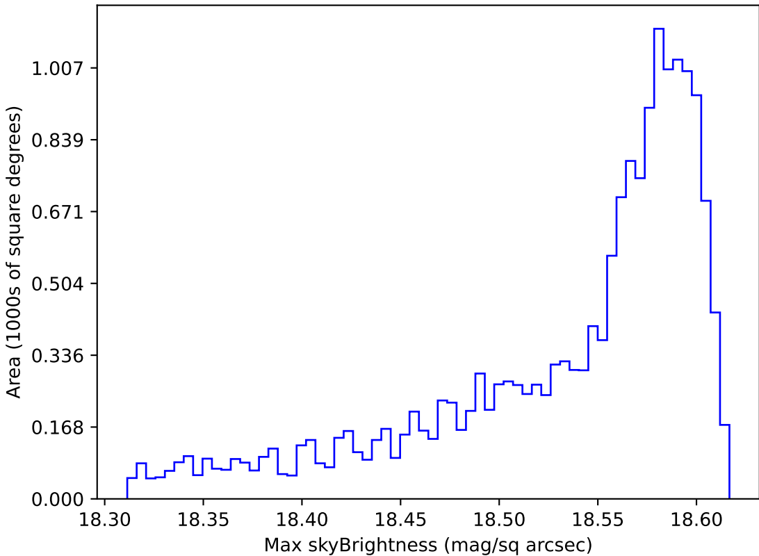
mw_roll_all_v3.3_10yrs WFD y band: Max skyBrightness
