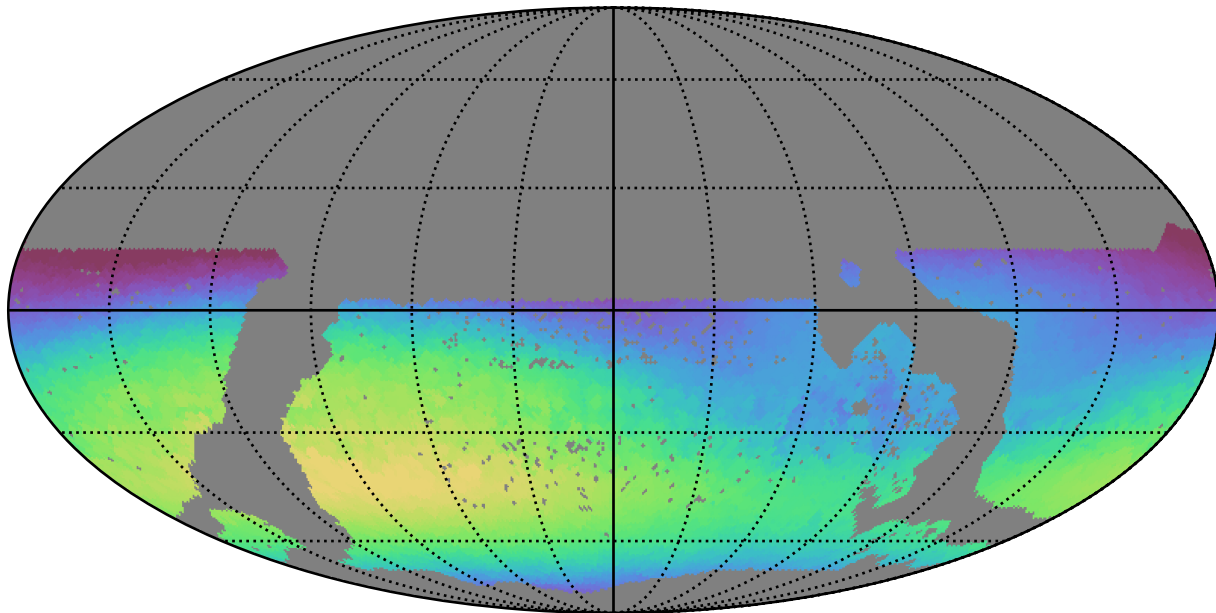
mw_roll_all_v3.3_10yrs WFD u band: Max skyBrightness
