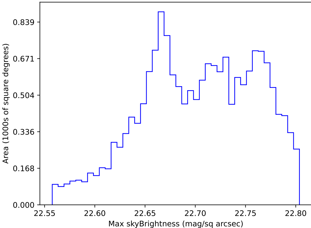
mw_roll_all_v3.3_10yrs WFD u band: Max skyBrightness
