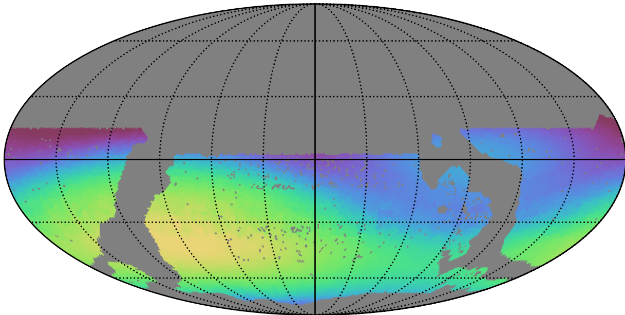
mw_roll_all_v3.3_10yrs WFD r band: Max skyBrightness
