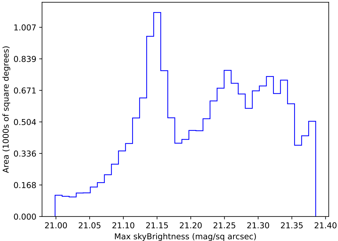
mw_roll_all_v3.3_10yrs WFD r band: Max skyBrightness
