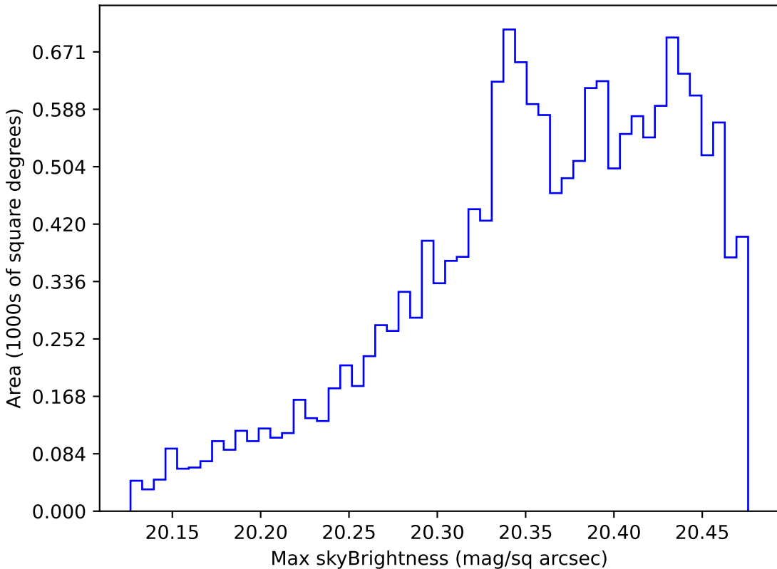
mw_roll_all_v3.3_10yrs WFD i band: Max skyBrightness
