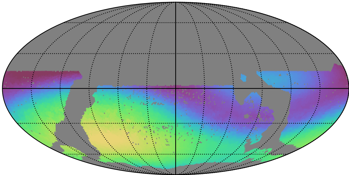
mw_roll_all_v3.3_10yrs WFD g band: Max skyBrightness
