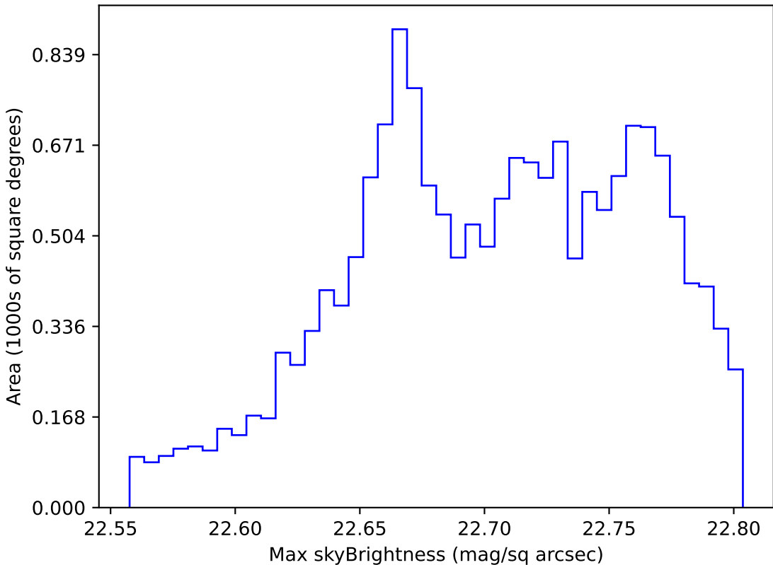
mw_roll_all_v3.3_10yrs WFD all bands: Max skyBrightness
