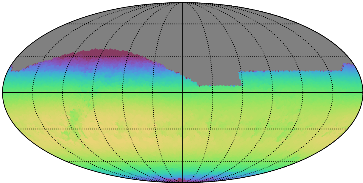
mw_roll_all_v3.3_10yrs All sky z band: Max skyBrightness
