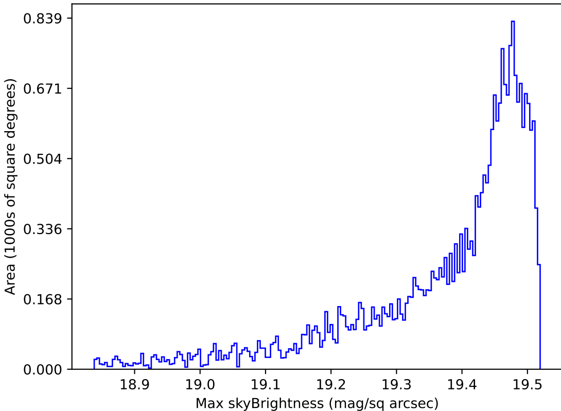
mw_roll_all_v3.3_10yrs All sky z band: Max skyBrightness
