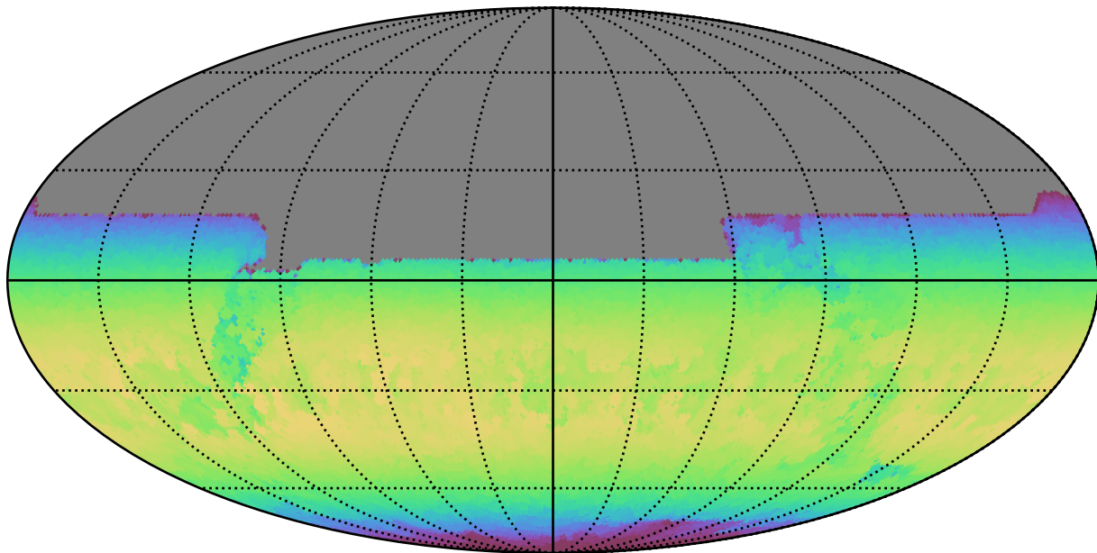
mw_roll_all_v3.3_10yrs All sky y band: Max skyBrightness
